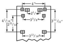
Rear Mount
